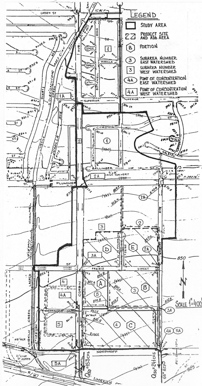
SOURCE: Drainage Study, 19601 Nordhoff Street, September, 2002. GM Engineering
