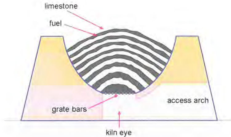
Figure 7 Cross-Section of Typical Pot-Kiln
