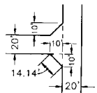
STANDARD CUT-CORNERS FOR 90° INTERSECTION (Plan View)
