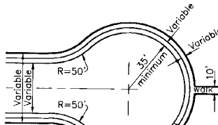
CUL-DE-SAC (Plan View)
