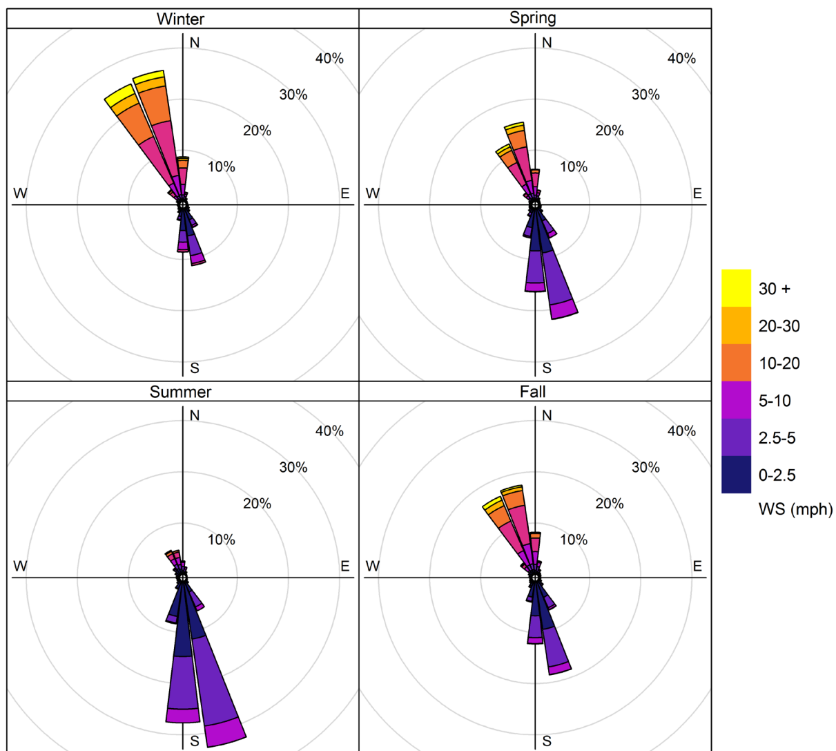
Figure B-4. Seasonal wind roses of hourly data collected at the Landfill monitor during 2007-2018.
