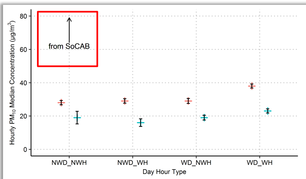
Figure 5-14. Year 11 (2018) hourly PM 10 median concentrations for northerly (“From SoCAB”) wind sectors (as displayed in Figure 5-4) for working days (WD) and non-working days (NWD) and for working hours (WH) and non-working hours (NWH) within those days for the Landfill (red) and Community (blue) monitor sites. 95% confidence intervals are shown in black.
