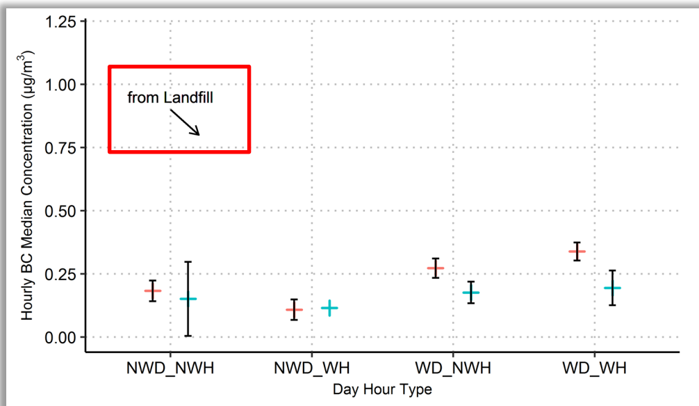
Figure 5-22. Year 11 (2018) hourly median BC concentrations for northerly (“From Landfill”) wind sectors (as displayed in Figure 5-4) for working days (WD) and non-working days (NWD) and for working hours (WH) and non-working hours (NWH) within those days for the Landfill (red) and Community (blue) monitor sites. 95% confidence intervals are shown in black.
