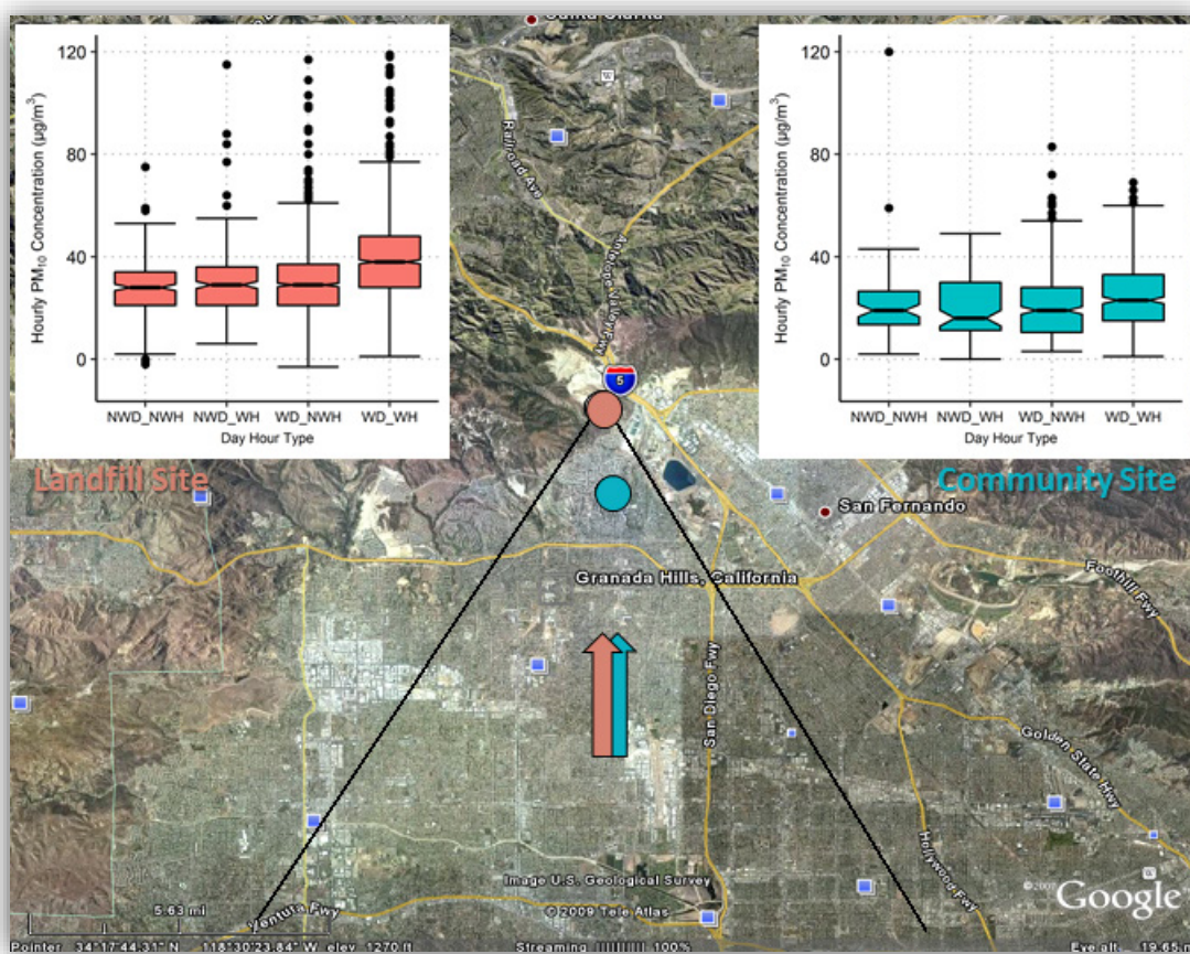
Figure 5-10. Notched box whisker plots of Year 11 (2018) hourly PM 10 concentrations for Southerly (“From SoCAB”) wind sectors (as displayed in Figure 5-4) for working days (WD) and non-working days (NWD) and for working hours (WH) and non-working hours (NWH) within those days for the Landfill (red) and Community (blue) monitor sites. Outliers over 120 µg/m 3 are not displayed.
