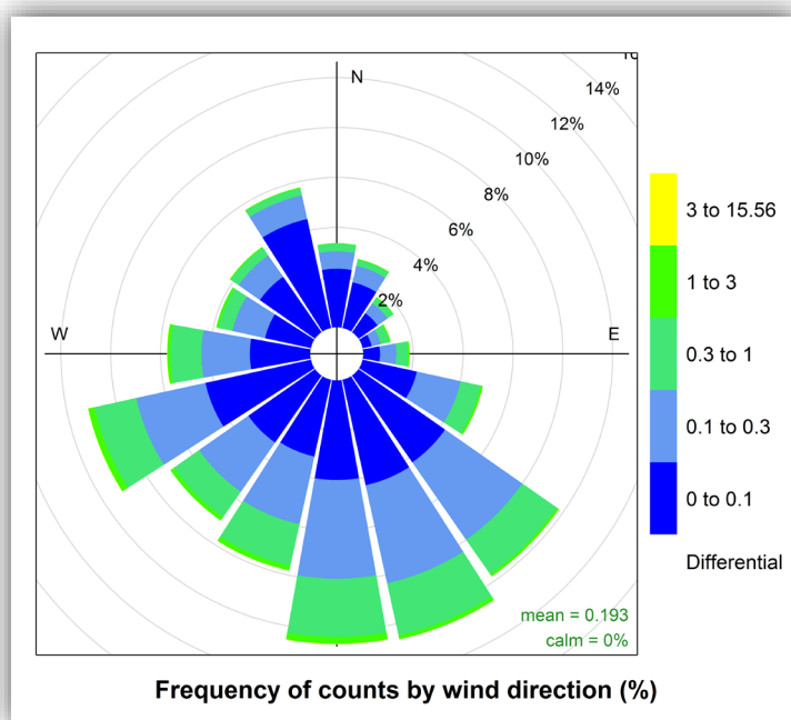
Figure 5-3. Black carbon pollution roses for the Community site showing the directions associated with highest BC concentrations (top) and the directions associated with BC concentrations that are higher than those at the Landfill site (bottom). Data are from December 7, 2007, through November 21, 2018.
