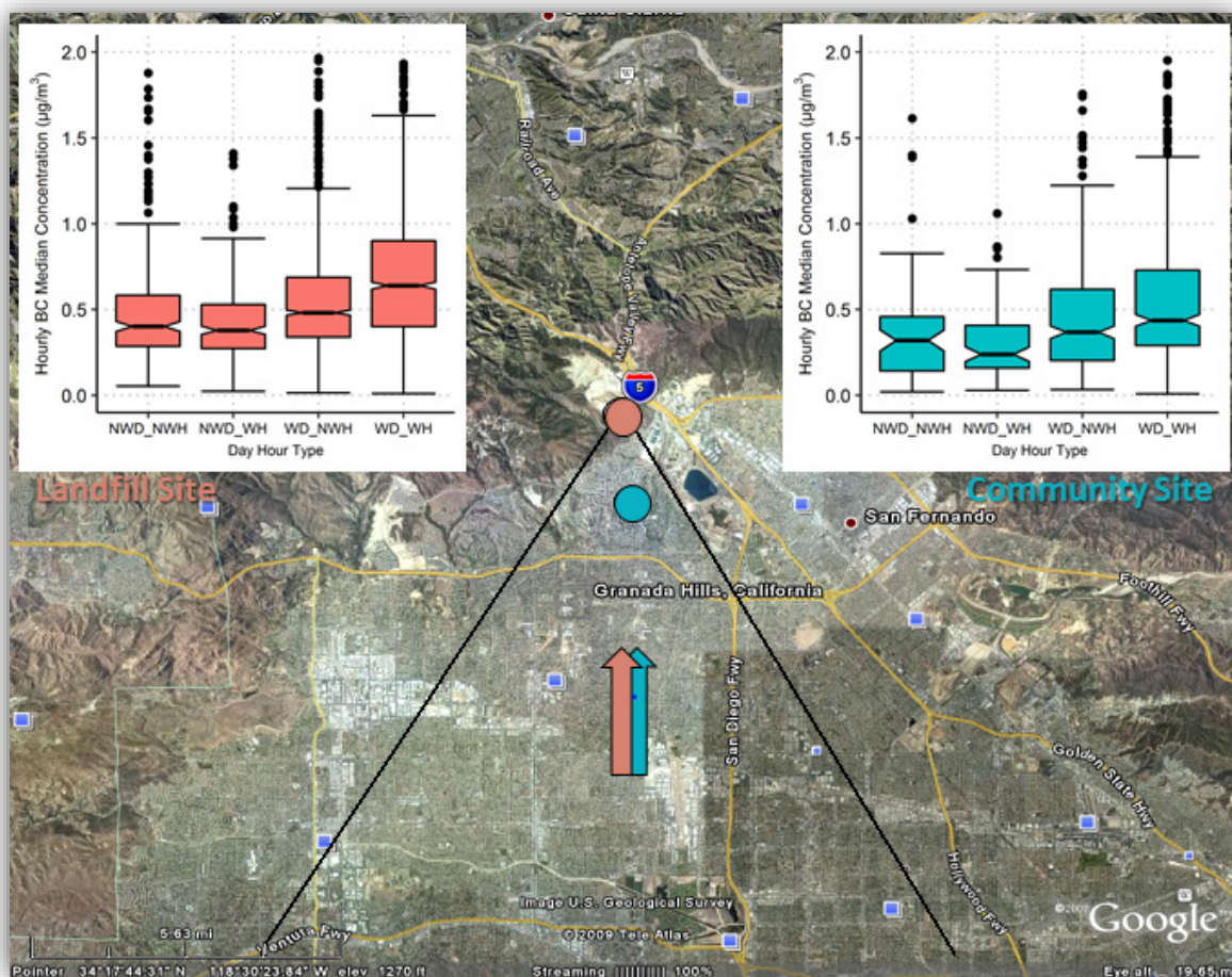
Figure 5-19. Notched box whisker plots of Year 11 (2018) hourly average BC concentrations for Southerly (“From SoCAB”) wind sectors (as displayed in Figure 5-4) for working days (WD) and non-working days (NWD) and for working hours (WH) and non-working hours (NWH) within those days for the Landfill (red) and Community (blue) monitor sites. Outliers over 2 µg/m³ are not displayed.
