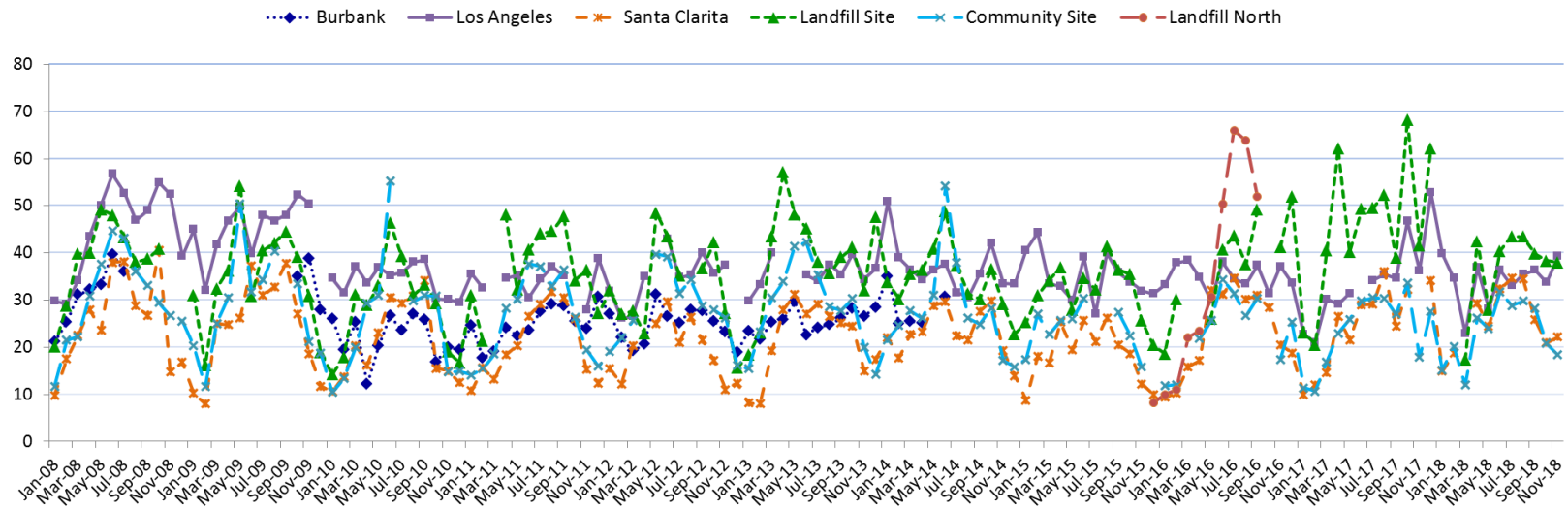
Figure 4-1. Monthly average PM 10 concentrations for the Landfill, Landfill North, and Community sites, and three regional monitoring sites for 2008–2018. (Notes: Like the Landfill and Community sites, Burbank and Los Angeles sites report hourly concentrations, while the Santa Clarita site reports integrated 24-hr samples on filters on a one-in-six day schedule. As of June 30, 2014, the Burbank site is no longer actively reporting PM 10 data. For the Landfill North site, the figure shows data through Nov. 21, 2017.)
