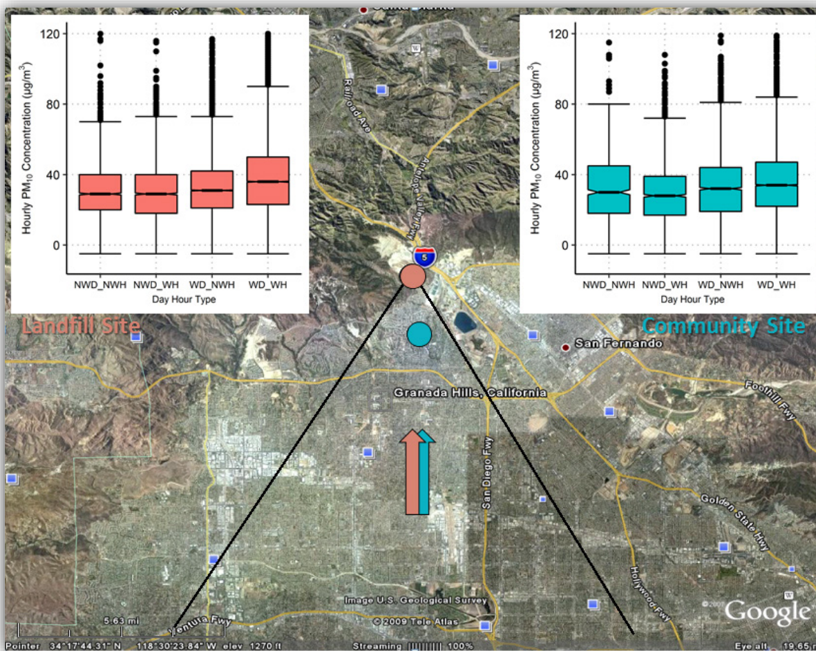
Figure 5-8. Notched box whisker plots of 11-year hourly PM 10 concentrations for southerly (“From SoCAB”) wind sectors (as displayed in Figure 5-4) for working days (WD) and non-working days (NWD) and for working hours (WH) and non-working hours (NWH) within those days for the Landfill (red) and Community (blue) monitor sites. Outliers over 120 μg/m 3 are not displayed.
