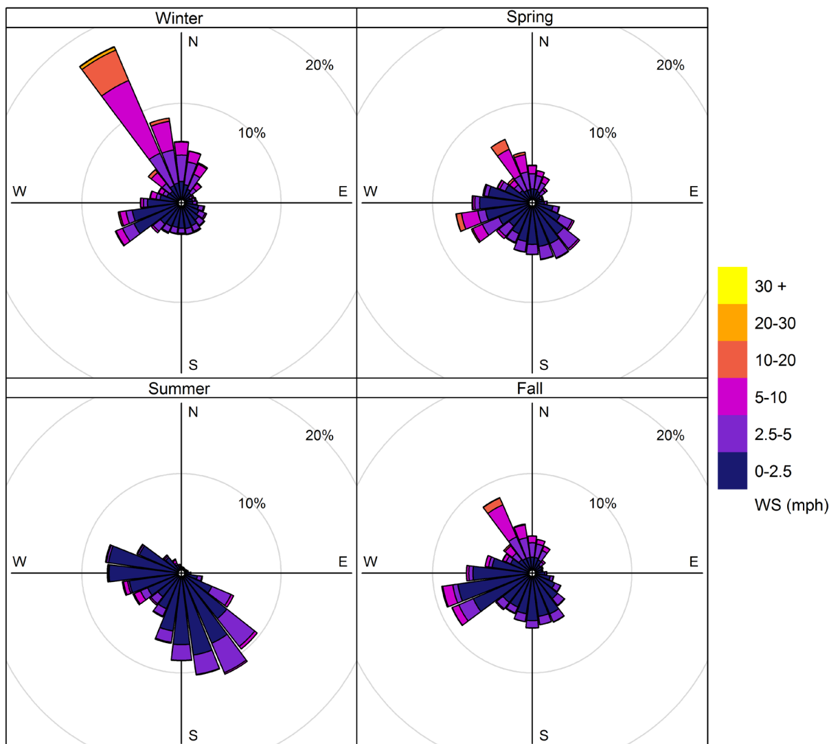
Figure B-5. Seasonal wind roses of hourly data collected at the Community monitor during 2007-2018.
