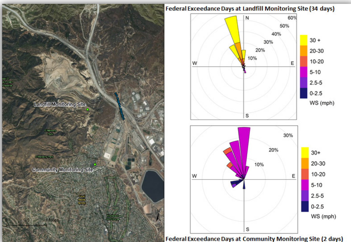
Figure 3-2. Wind rose from federal exceedance days during 11 continuous monitoring years at the Landfill (top right) and Community (bottom right) monitoring sites.
