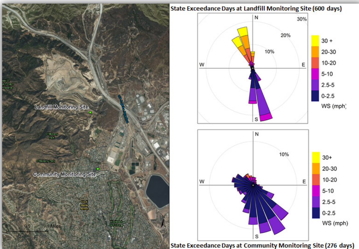
Figure 3-4. Wind rose from state 24-hr PM 10 exceedance days during 11 continuous monitoring years at the Landfill (top right) and Community (bottom right) monitoring sites.
