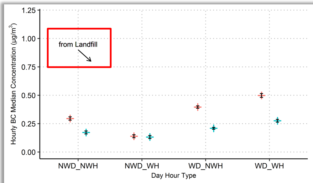
Figure 5-20. Eleven-year hourly median BC concentrations for northerly (“From Landfill”) wind sectors (as displayed in Figure 5-4) for working days (WD) and non-working days (NWD) and for working hours (WH) and non-working hours (NWH) within those days for the Landfill (red) and Community (blue) monitor sites. 95% confidence intervals are shown in black.
