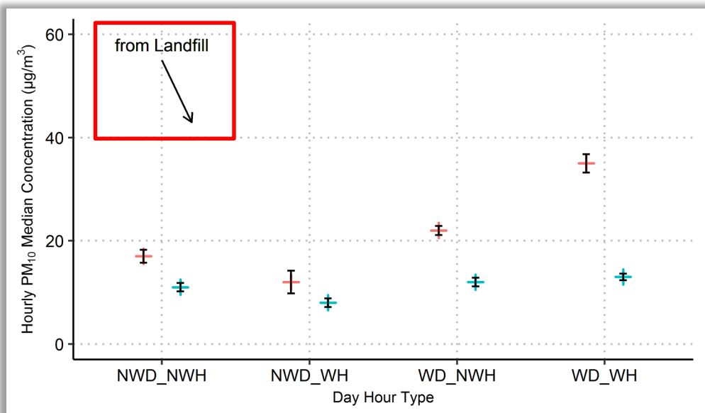
Figure 5-11. Eleven-year hourly PM 10 median concentrations for northerly (“From Landfill”) wind sectors (as displayed in Figure 5-4) for working days (WD) and non-working days (NWD) and for working hours (WH) and non-working hours (NWH) within those days for the Landfill (red) and Community (blue) monitor sites. 95% confidence intervals are shown in black.
