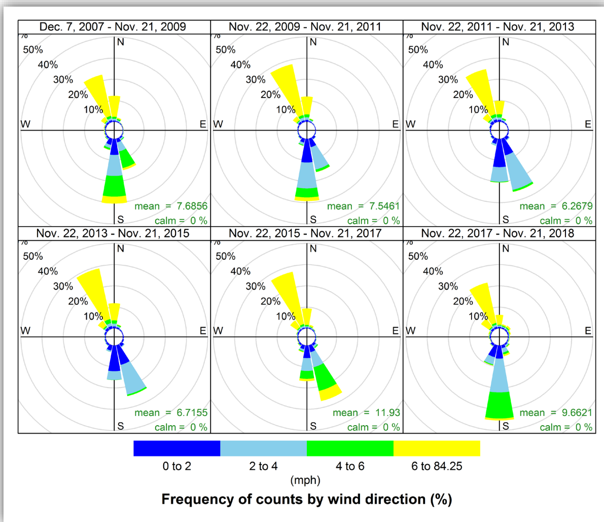
Figure 5-1. Landfill station wind roses over the 11 years of monitoring data. Winds are highly directional at the Landfill site. Wind data for monitoring Years 1 through 10 are shown in two-year groups in the first five wind roses (top three, bottom left, and bottom center), while the data for Year 11 are displayed in an individual wind rose (bottom right).
