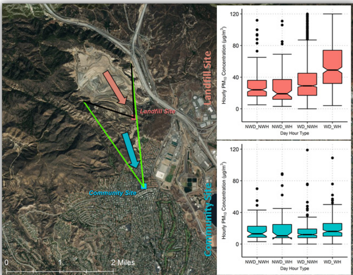
Figure 5-9. Notched box whisker plots of Year 11 (2018) hourly PM 10 concentrations for northerly (“From Landfill”) wind sectors (as displayed in Figure 5-4) for working days (WD) and non-working days (NWD) and for working hours (WH) and non-working hours (NWH) within those days for the Landfill (red) and Community (blue) monitor sites. Outliers over 120 µg/m 3 are not displayed.
