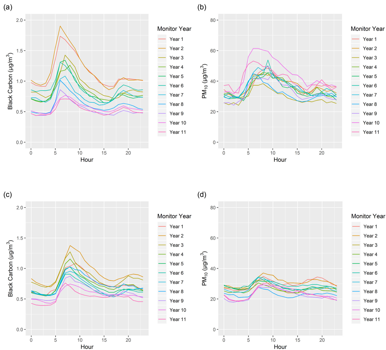
Figure B-1. Mean BC and PM 10 concentrations by hour for the 11 monitoring years at the Landfill (a, b) and Community (c, d) sites.
