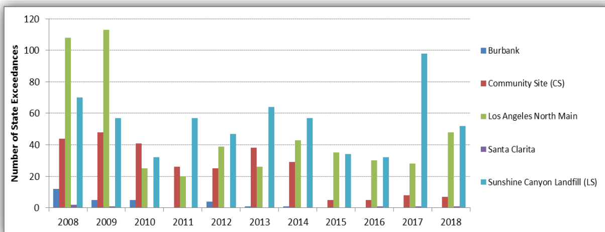
Figure 3-3. Number of state exceedances of 24-hr PM 10 at the Landfill, Community, and regional monitoring sites by year over the 11-year study period.
