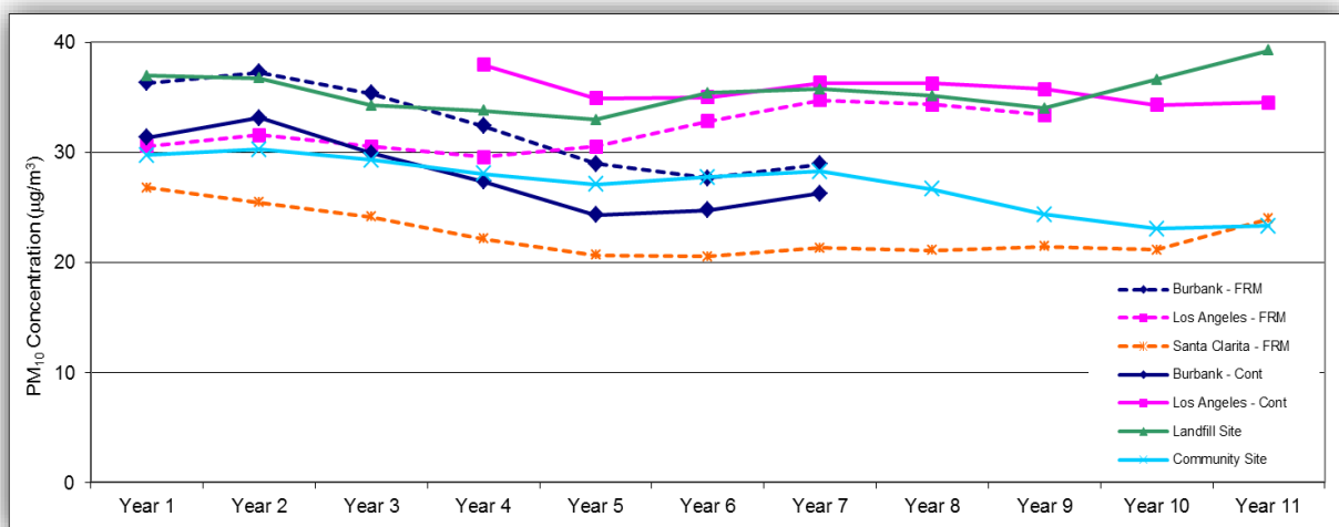
Figure 4-2. Rolling annual average PM 10 concentrations for the Landfill and Community sites, and three regional monitoring sites for 2008–2018.
