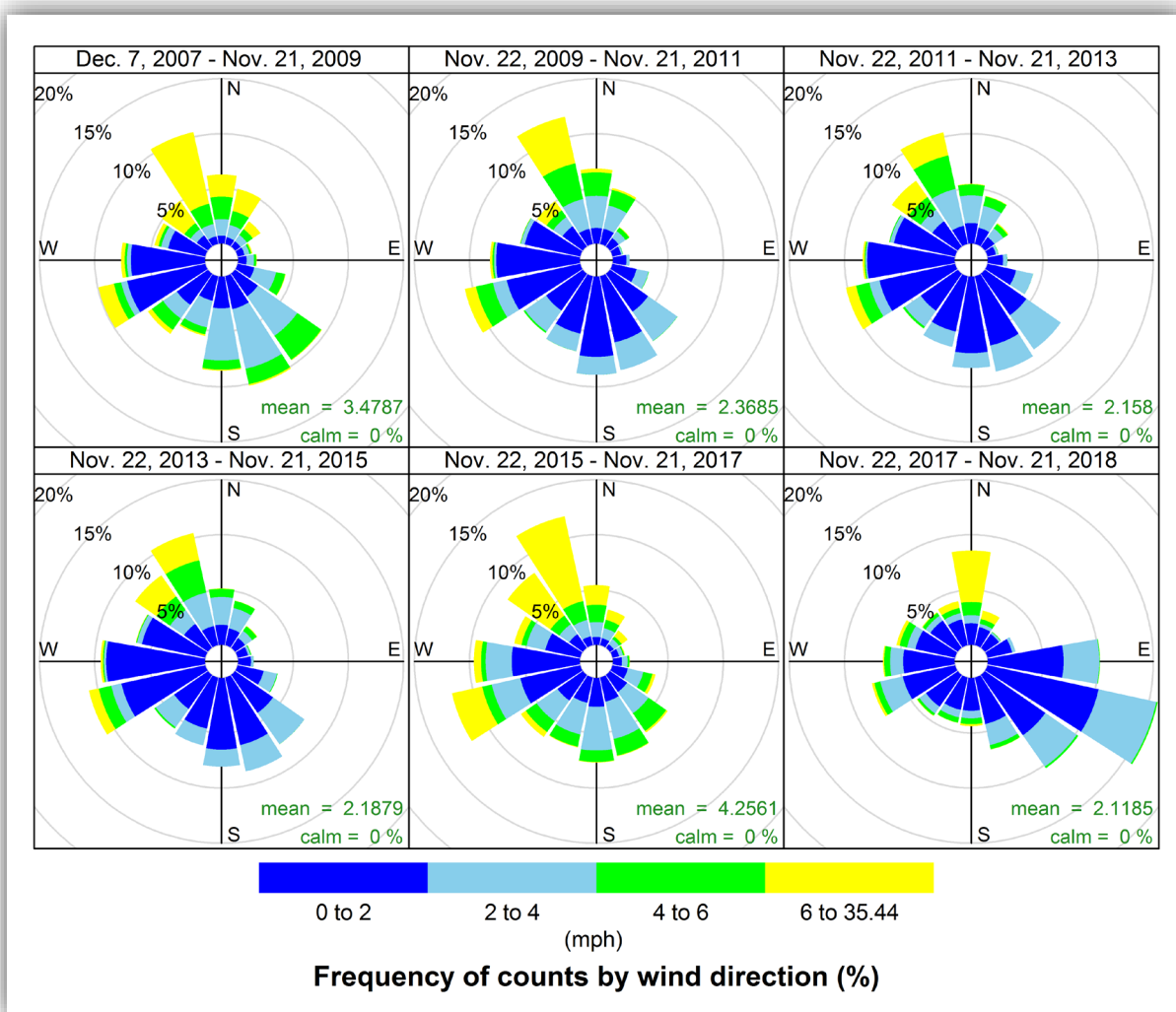
Figure 5-2. Community site wind roses over the 11 years of monitoring data. Winds are more variable at the Community site than at the Landfill site. Wind data for monitoring Years 1 through 10 are shown in two-year groups in the first five wind roses (top three, bottom left, and bottom), while the data for Year 11 (Reseda site) are displayed in an individual wind rose (bottom right).
