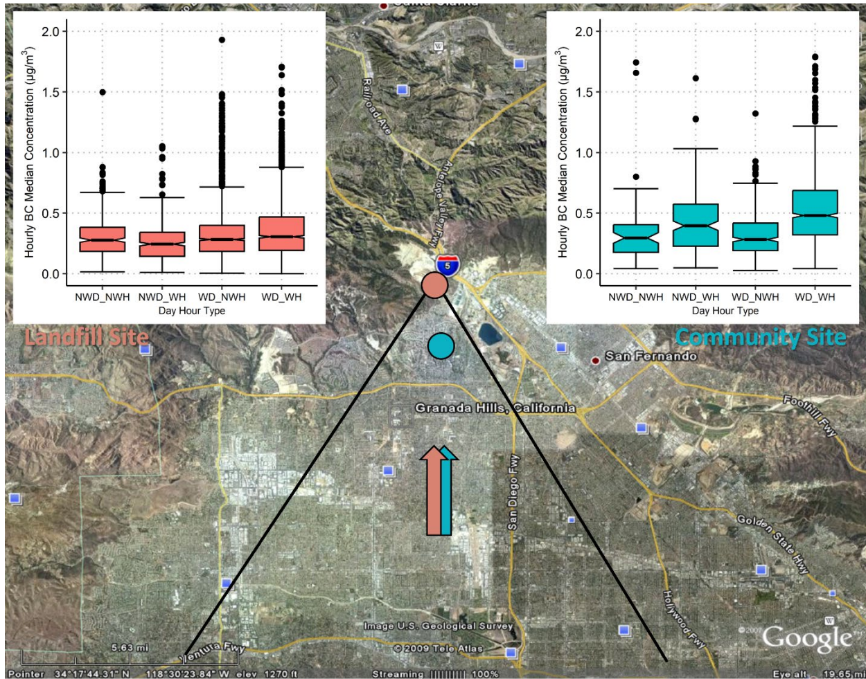
Figure 5-19. Notched box whisker plots of Year 18 (2025) hourly average BC concentrations for southerly ("From SoCAB") wind sectors (as displayed in Figure 5-5) for working days (WD), non-working days (NWD), working hours (WH), and non-working hours (NWH) within those days for the Landfill (red) and Community (blue) monitor sites. Outliers over 2 \mu\text{g}/\text{m}^3 are not displayed.
