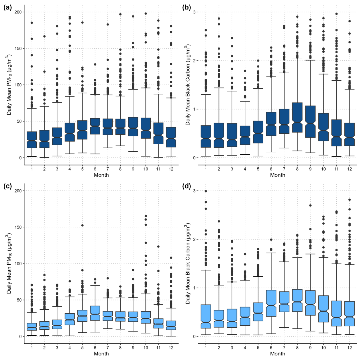
Figure B-2. Distribution of daily mean PM 10 and BC concentrations by month across all 18 monitor years (2007–2025) at the Landfill (a, b) and Community (c, d) sites. Note: BC outliers greater than 3 µg/m 3 and PM 10 outliers greater than 200 µg/m 3 are excluded.
