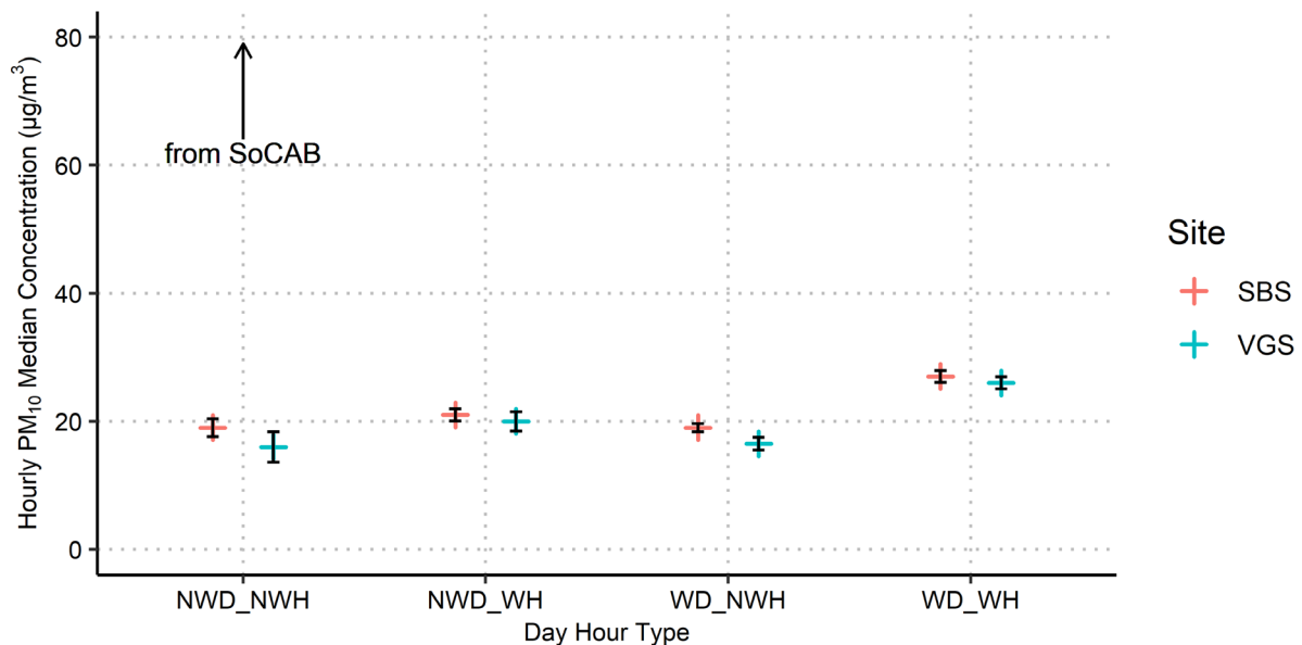
Figure 5-14. Year 18 (2025) hourly PM_{10} median concentrations for northerly (“From SoCAB”) wind sectors (as displayed in Figure 5-5) for working days (WD), non-working days (NWD), working hours (WH), and non-working hours (NWH) within those days for the Landfill (red) and Community (blue) monitor sites. 95% confidence intervals are shown in black.
