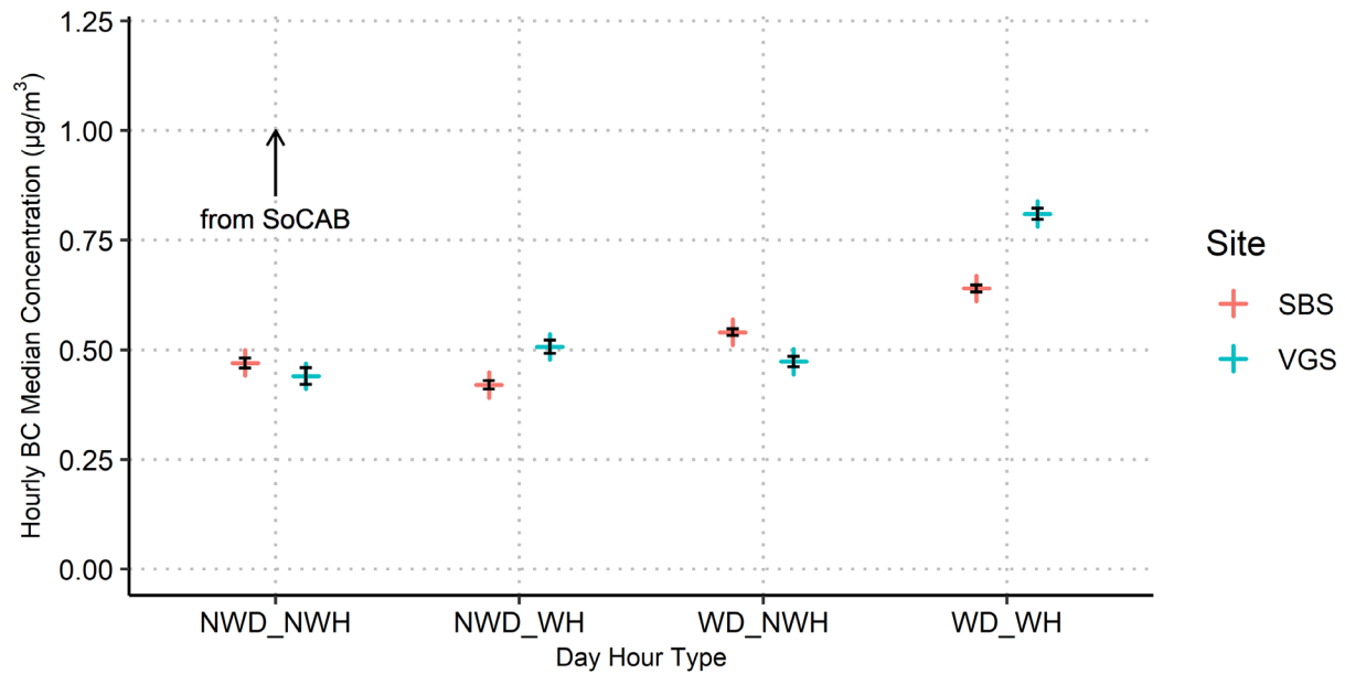
Figure 5-21. Eighteen-yr hourly median BC concentrations for northerly ("From SoCAB") wind sectors (as displayed in Figure 5-5) for working days (WD), non-working days (NWD), working hours (WH), and non-working hours (NWH) within those days for the Landfill (red) and Community (blue) monitor sites. 95% confidence intervals are shown in black.
