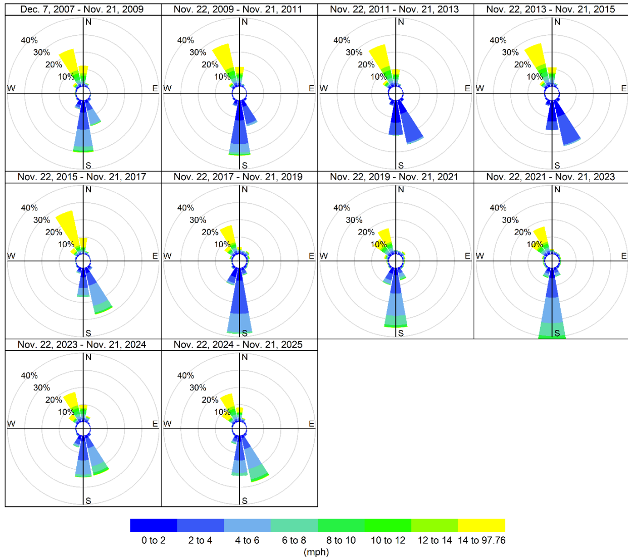
Figure 5-1. Wind roses for the Landfill site over the 18 years of monitoring data. Wind data for monitoring Years 1 through 16 are shown in 2-yr groups, while the data for Year 17 through Year 18 are displayed as individual wind roses. Only data labeled “valid” or “suspect” are used.
