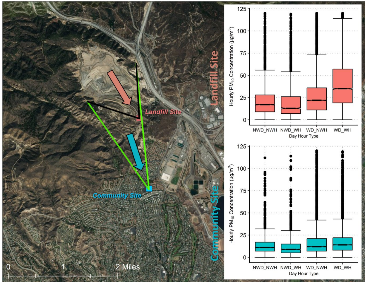
Figure 5-7. Notched box whisker plots of 18-yr hourly PM_{10} concentrations for northerly ("From Landfill") wind sectors (as displayed in Figure 5-4) for working days (WD), non-working days (NWD), working hours (WH), and non-working hours (NWH) within those days for the Landfill (red) and Community (blue) monitor sites. Outliers over 125 \mu g/m^3 are not displayed.
