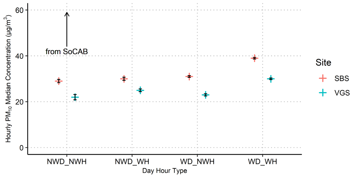
Figure 5-12. Eighteen-yr hourly PM_{10} median concentrations for northerly ("From SoCAB") wind sectors (as displayed in Figure 5-5) for working days (WD), non-working days (NWD), working hours (WH), and non-working hours (NWH) within those days for the Landfill (red) and Community (blue) monitor sites. 95% confidence intervals are shown in black.
