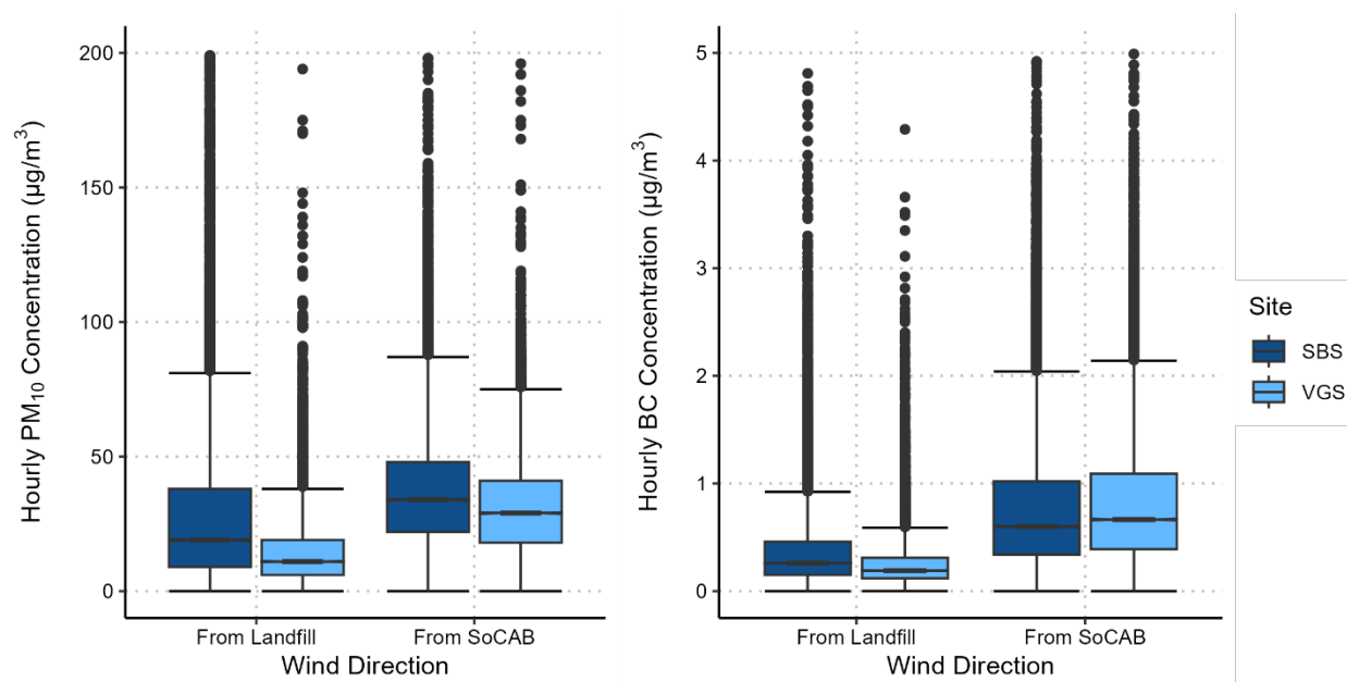
Figure B-7. PM 10 (left) and BC (right) concentrations at the Landfill (dark blue) and Community (light blue) sites from November 22, 2007, through November 21, 2025, when winds originated from the Landfill versus when they originated from the SoCAB. Results are based on hourly data points where both sites experienced winds from the same sector. Note that BC data greater than 5 µg/m 3 and PM 10 data greater than 200 µg/m 3 are excluded.
