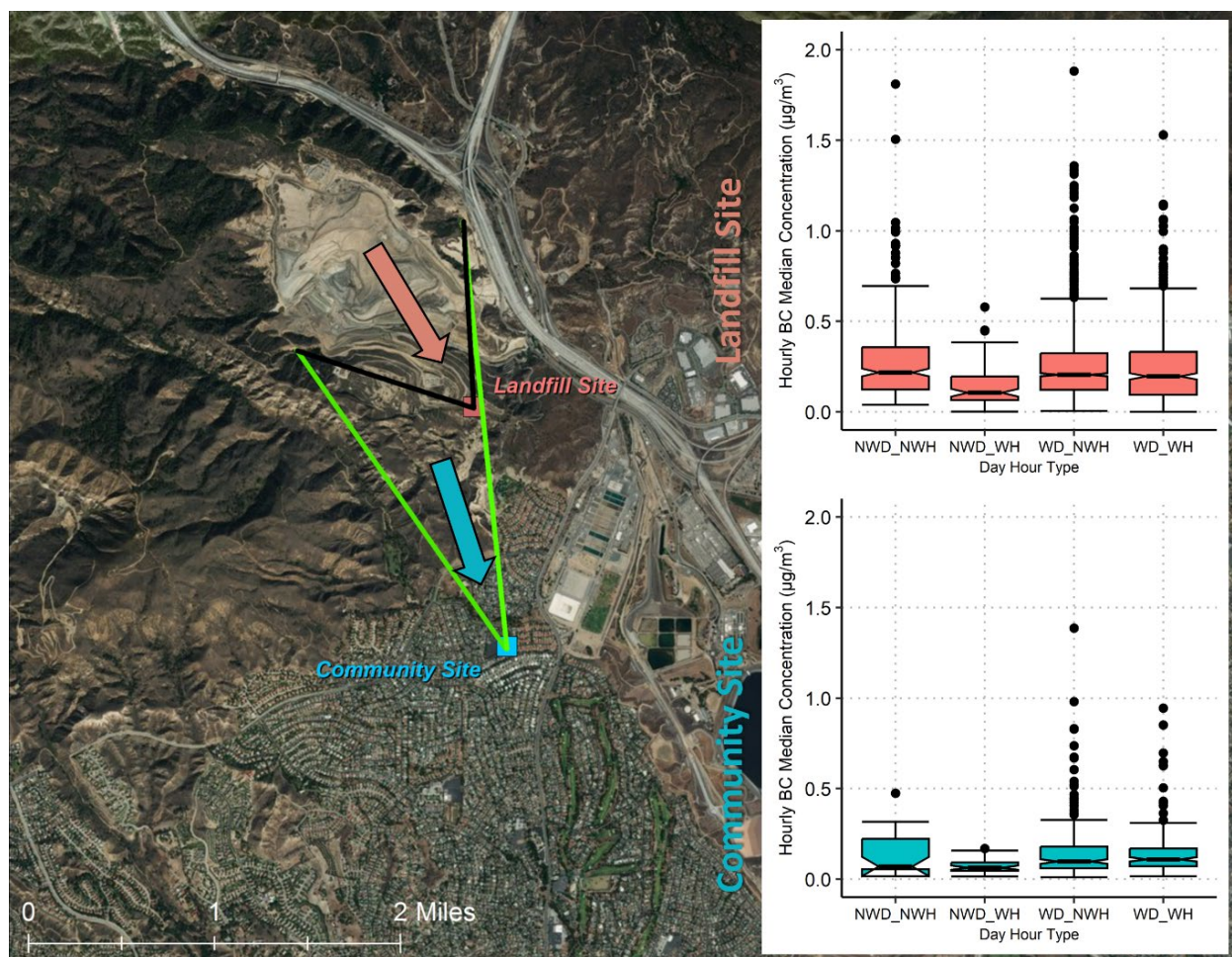
Figure 5-18. Notched box whisker plots of Year 18 (2025) hourly average BC concentrations for northerly ("From Landfill") wind sectors (as displayed in Figure 5-4) for working days (WD), non-working days (NWD), working hours (WH), and non-working hours (NWH) within those days for the Landfill (red) and Community (blue) monitor sites. Outliers over 2 \mu\text{g}/\text{m}^3 are not displayed.
