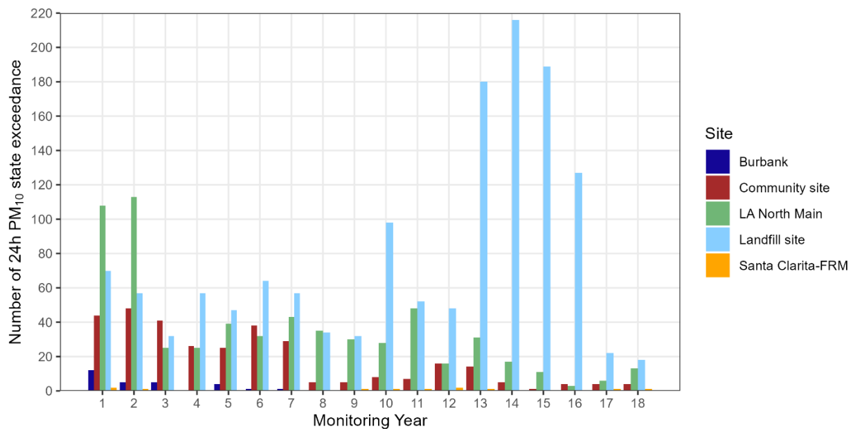
Figure 3-5. Number of state exceedances of 24-hr PM_{10} at the Landfill, Community, and regional monitoring sites by year over the 18-yr study period. (e.g., Monitoring Year 1 refers to Nov. 22, 2007–Nov. 21, 2008).
