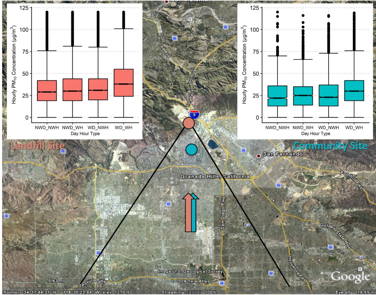
Figure 5-8. Notched box whisker plots of 18-yr hourly PM_{10} concentrations for southerly ("From SoCAB") wind sectors (as displayed in Figure 5-5) for working days (WD), non-working days (NWD), working hours (WH), and non-working hours (NWH) within those days for the Landfill (red) and Community (blue) monitor sites. Outliers over 125 \mu g/m^3 are not displayed.
