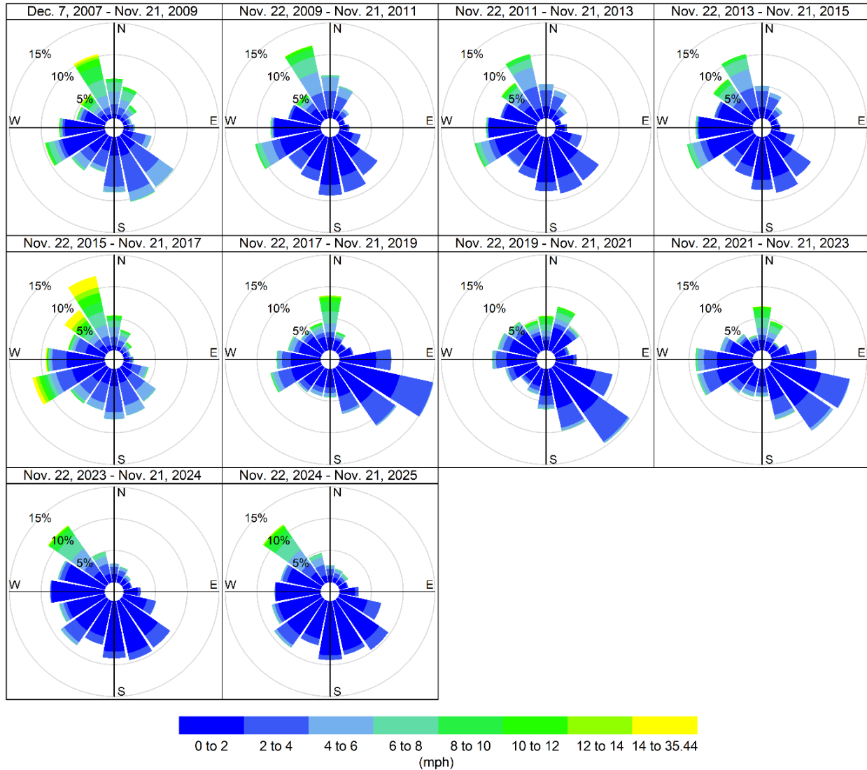
Figure 5-2. Wind roses for the Community Site over the 18 years of monitoring data. Wind data for monitoring Years 1 through 16 are shown in 2-yr groups, while the data for Year 17 through Year 18 are displayed as individual wind roses. Only data labeled “valid” or “suspect” are used. Wind data at the Community site were replaced with those from the Reseda site from Year 11 to Year 16.
