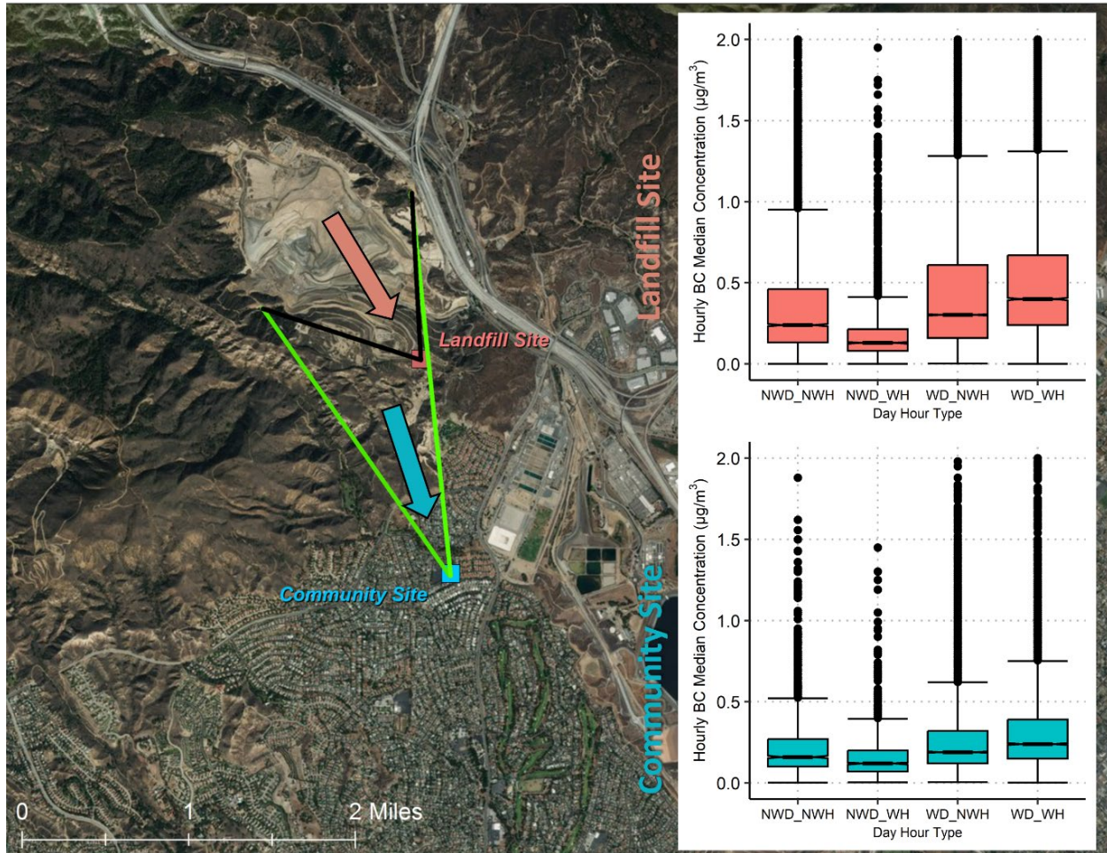
Figure 5-16. Notched box whisker plots of 18-yr hourly average BC concentrations for northerly ("From Landfill") wind sectors (as displayed in Figure 5-4) for working days (WD), non-working days (NWD), working hours (WH), and non-working hours (NWH) within those days for the Landfill (red) and Community (blue) monitor sites. Outliers over 2 \mu\text{g}/\text{m}^3 are not displayed.
