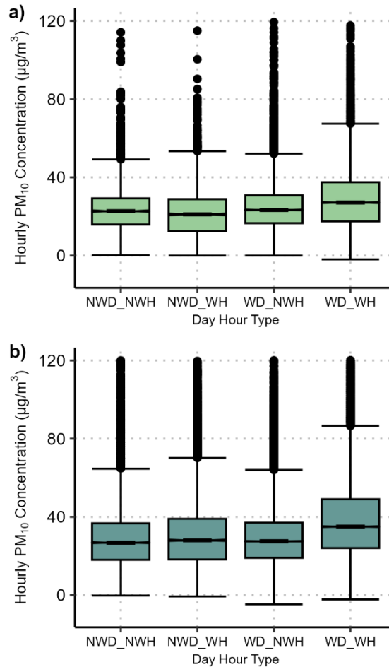
Figure 5-15. Hourly PM_{10} median concentrations for (a) Burbank (2008-2014) and (b) Los Angeles (2008-2025) for working days (WD), non-working days (NWD), working hours (WH), and non-working hours (NWH).
