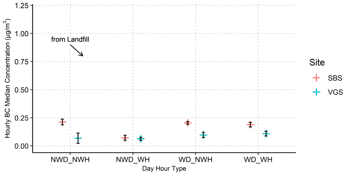
Figure 5-22. Year 18 (2025) hourly median BC concentrations for northerly ("From Landfill") wind sectors (as displayed in Figure 5-4) for working days (WD), non-working days (NWD), working hours (WH), and non-working hours (NWH) within those days for the Landfill (red) and Community (blue) monitor sites. 95% confidence intervals are shown in black.
