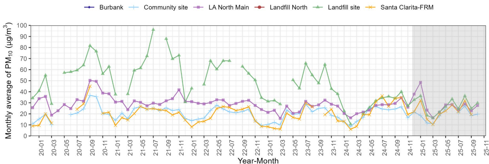
Figure 4-2. Monthly average PM 10 concentrations for the Landfill and Community sites, and three regional monitoring sites from Year 13 through Year 18. The Santa Clarita site reports integrated 24-hr samples of filters on a one-in-six-day schedule. The current year (Year 18) time period is shaded in grey.
