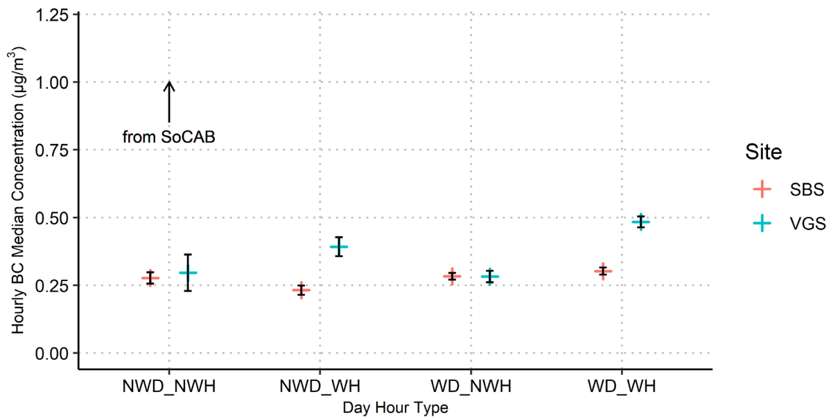
Figure 5-23. Year 18 (2025) hourly median BC concentrations for northerly ("From SoCAB") wind sectors (as displayed in Figure 5-5) for working days (WD), non-working days (NWD), working hours (WH), and non-working hours (NWH) within those days for the Landfill (red) and Community (blue) monitor sites. 95% confidence intervals are shown in black.
