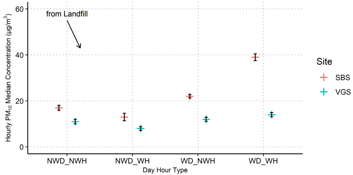
Figure 5-11. Eighteen-yr hourly PM_{10} median concentrations for northerly ("From Landfill") wind sectors (as displayed in Figure 5-4) for working days (WD), non-working days (NWD), working hours (WH), and non-working hours (NWH) within those days for the Landfill (red) and Community (blue) monitor sites. 95% confidence intervals are shown in black.
