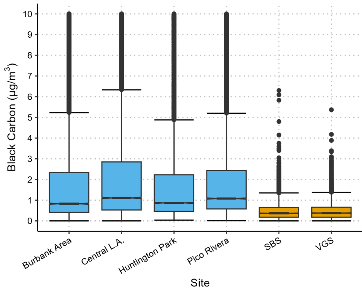
Figure A-2. A comparison of regional BC concentrations from May 2018 through April 2019 at landfill sites (yellow) and MATES V monitoring stations (blue). In MATES V documentation, Los Angeles is referred to as “Central L.A.” and Burbank is referred to as “Burbank Area”. Note that outliers above 10 \mu\text{g}/\text{m}^3 are excluded.
