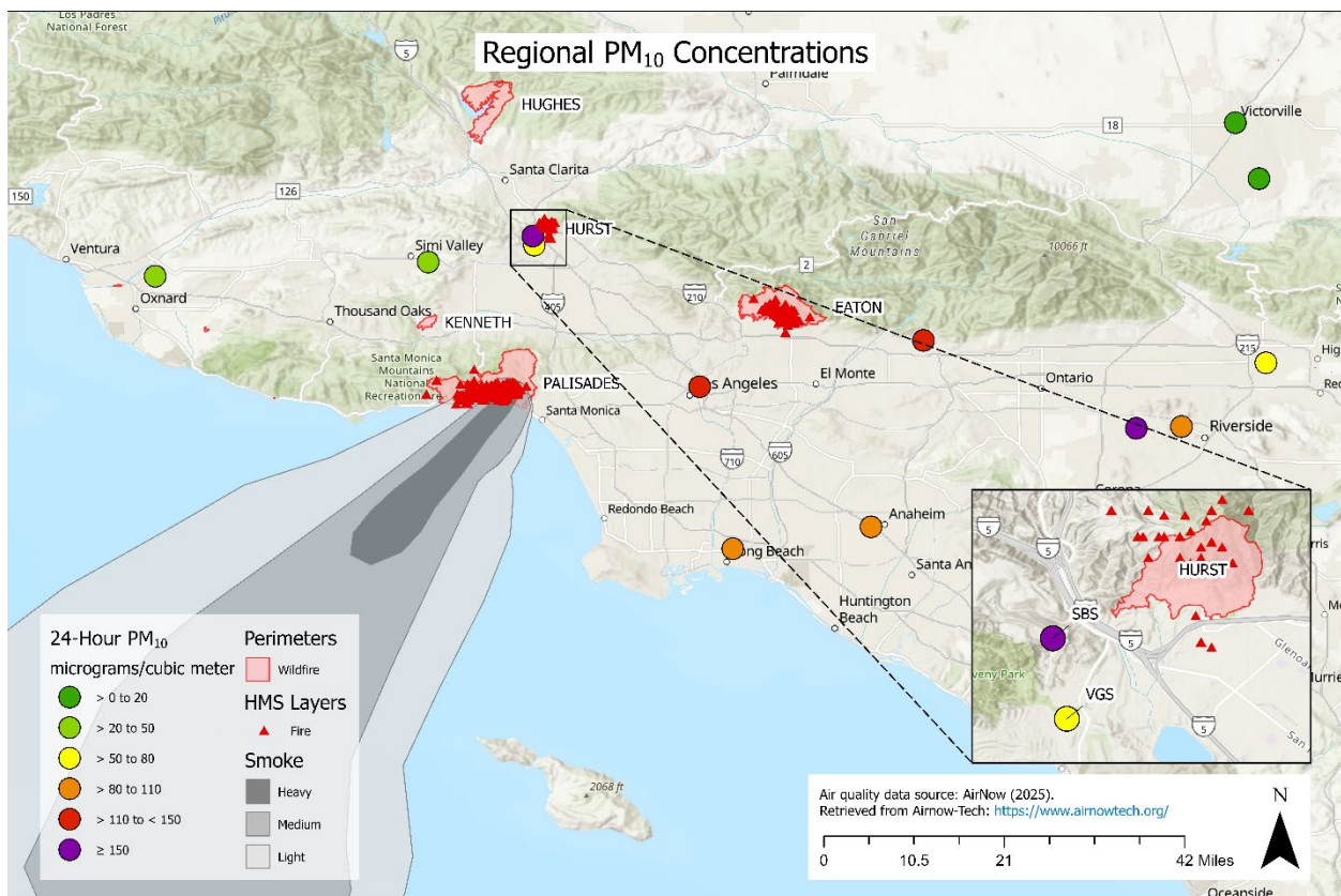
Figure 3-2. PM 10 concentrations at air monitoring sites across the Los Angeles area on January 7, 2025. Colors correspond to 24-hr PM 10 concentrations in µg/m 3 . HMS fire and smoke layers from January 7, 2025, the day of the exceedance, and fire perimeters from January 7, 2025, are overlaid. Note: only the Palisades, Hurst, and Eaton fires were actively burning on January 7, 2025.
