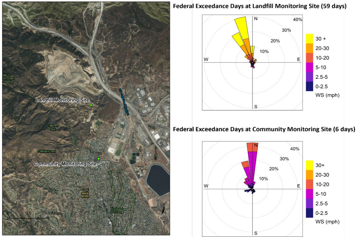
Figure 3-4. Wind rose from federal exceedance days during 18 continuous monitoring years at the Landfill (top right) and Community (bottom right) sites. Wind data at the Community site are replaced with those from the Reseda site from Year 11 to Year 16.
