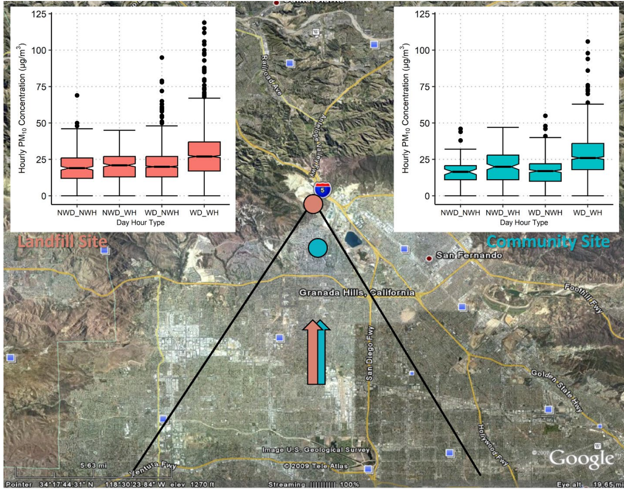
Figure 5-10. Notched box whisker plots of Year 18 (2025) hourly PM_{10} concentrations for southerly ("From SoCAB") wind sectors (as displayed in Figure 5-5) for working days (WD), non-working days (NWD), working hours (WH), and non-working hours (NWH) within those days for the Landfill (red) and Community (blue) monitor sites. Outliers over 125 \mu g/m^3 are not displayed.
