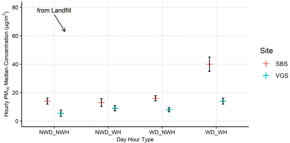
Figure 5-13. Year 18 (2025) hourly PM_{10} median concentrations for northerly (“From Landfill”) wind sectors (as displayed in Figure 5-4) for working days (WD), non-working days (NWD), working hours (WH), and non-working hours (NWH) within those days for the Landfill (red) and Community (blue) monitor sites. 95% confidence intervals are shown in black. Note that confidence intervals are a function of the number of data points; fewer data points lead to a wider interval and less certainty about where the median falls.
