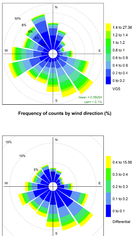
Figure 5-3. Top panel: pollution rose of hourly BC concentration at the Community site. Bottom panel: pollution differential rose of excess hourly BC concentration at the Community site (compared to the Landfill site). Data are from December 7, 2007, through November 21, 2025. Data are used only when both BC and wind direction are labeled “valid.”
