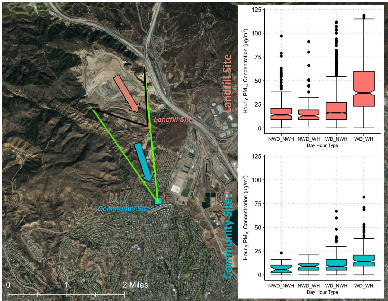
Figure 5-9. Notched box whisker plots of Year 18 (2025) hourly PM_{10} concentrations for northerly (“From Landfill”) wind sectors (as displayed in Figure 5-4) for working days (WD), non-working days (NWD), working hours (WH), and non-working hours (NWH) within those days for the Landfill (red) and Community (blue) monitor sites. Outliers over 125 \mu g/m^3 are not displayed.
