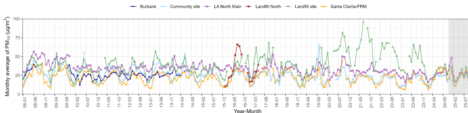
Figure 4-1. Monthly average PM 10 concentrations for the Landfill, Landfill North (in operation from June 2016 until May 2017), and Community sites, and three regional monitoring sites for 2008–2025. The Santa Clarita site reports integrated 24-hr samples of filters on a one-in-six-day schedule. As of June 30, 2014, the Burbank site is no longer actively reporting PM 10 data. The current year (Year 18) time period is shaded in grey.
