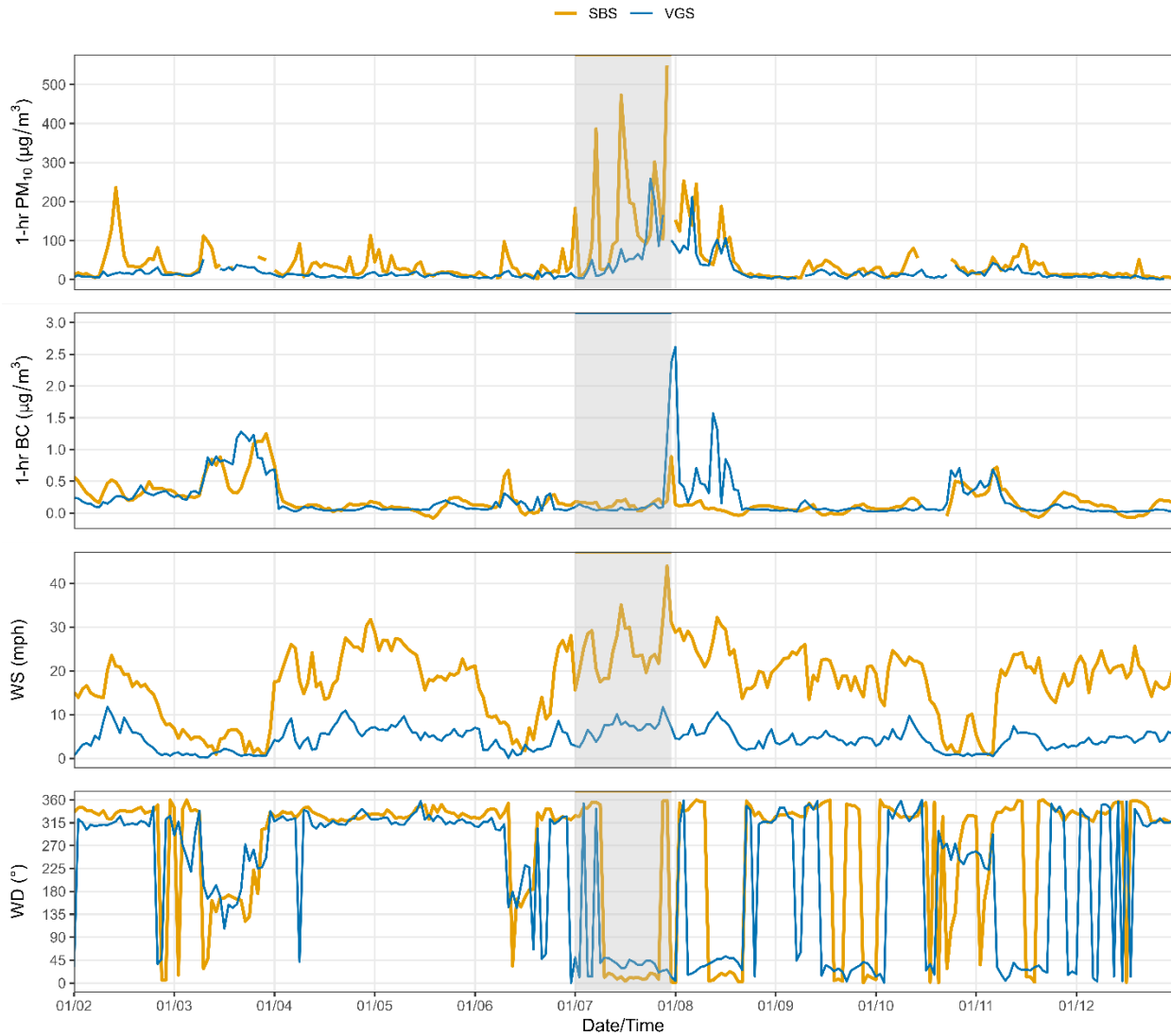
Figure 3-3. Hourly time series of PM_{10} and BC concentrations (top two rows) and WS/WD measurements (bottom two rows) recorded at the Landfill and Community sites five days before and after the January 7, 2025, PM_{10} exceedance at the Landfill site. The gray rectangle indicates January 7, 2025.
