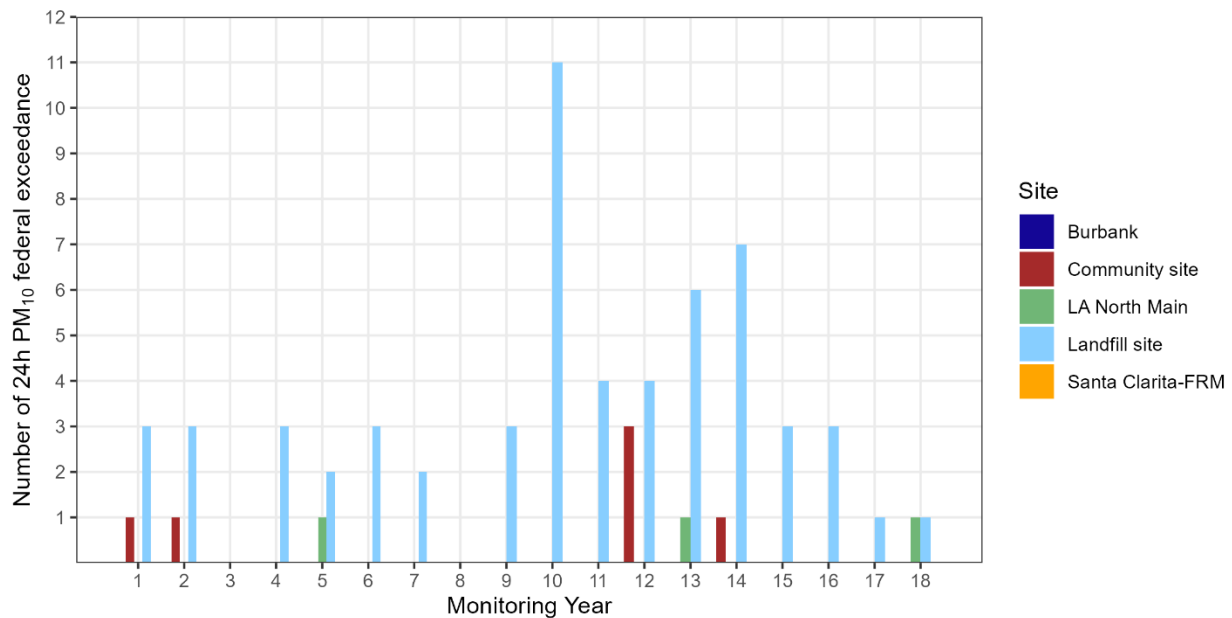
Figure 3-1. The number of federal exceedances of 24-hr PM_{10} at the Landfill, Community, and regional monitoring sites by year over the 18-yr study period. (e.g., Monitoring Year 1 refers to Nov. 22, 2007–Nov. 21, 2008).
