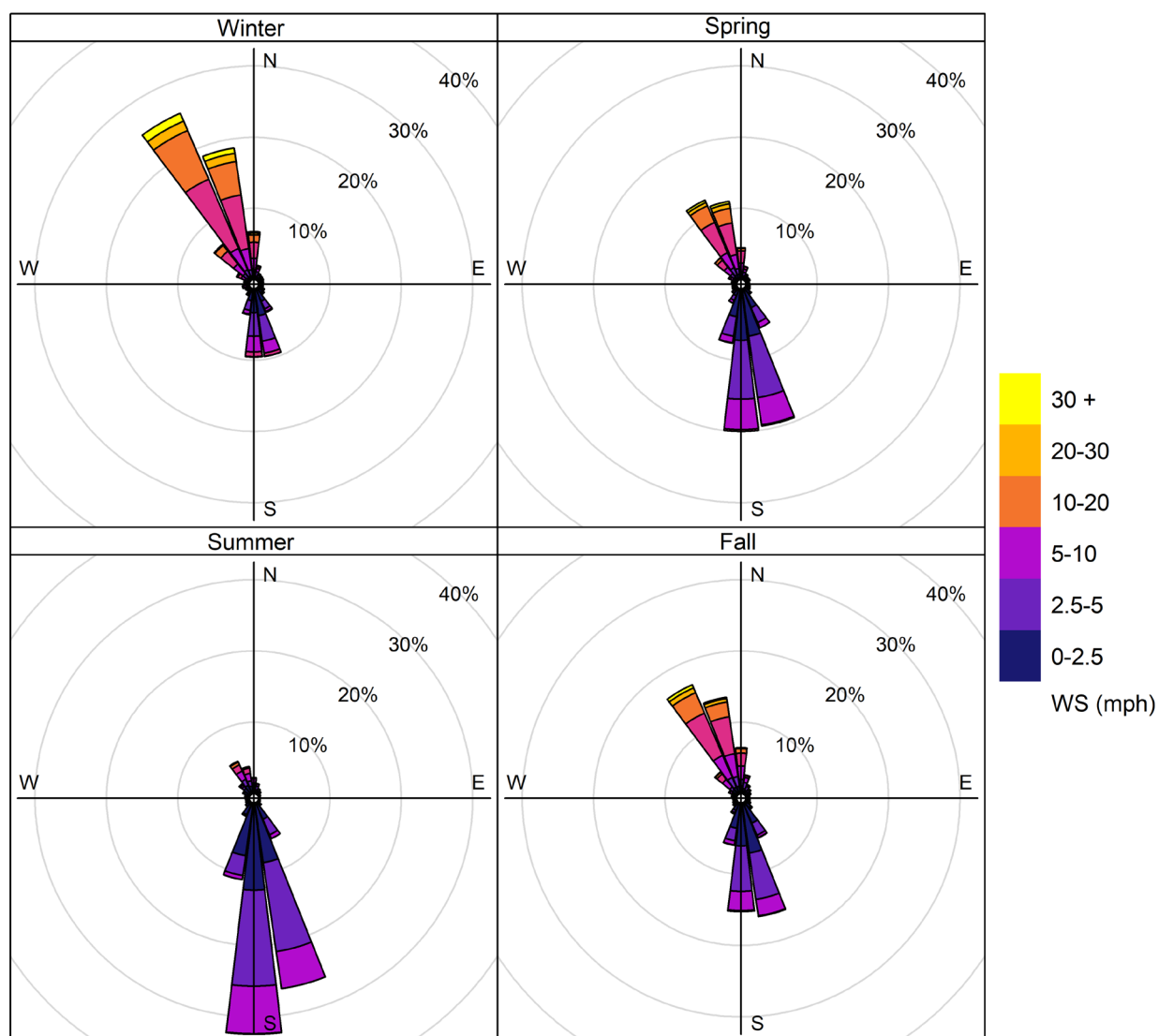
Figure B-4. Seasonal wind roses based on hourly data collected at the Landfill site from 2007-2025.
