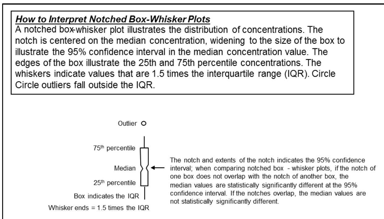
Figure 5-6. Instructions for interpreting notched box-whisker plots.
