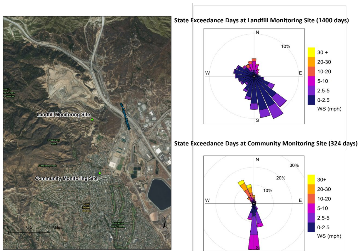
Figure 3-6. Wind rose from state 24-hr PM_{10} exceedance days during 18 continuous monitoring years at the Landfill (top right) and Community (bottom right) sites. Wind data at the Community site have been replaced with those from the Reseda site from Year 11 to Year 16 (as discussed in Section 5.1).
