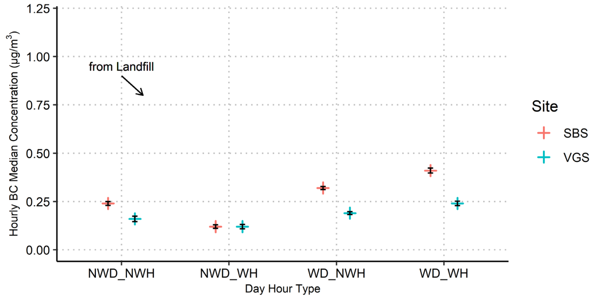
Figure 5-20. Eighteen-yr hourly median BC concentrations for northerly ("From Landfill") wind sectors (as displayed in Figure 5-4) for working days (WD), non-working days (NWD), working hours (WH), and non-working hours (NWH) within those days for the Landfill (red) and Community (blue) monitor sites. 95% confidence intervals are shown in black.
