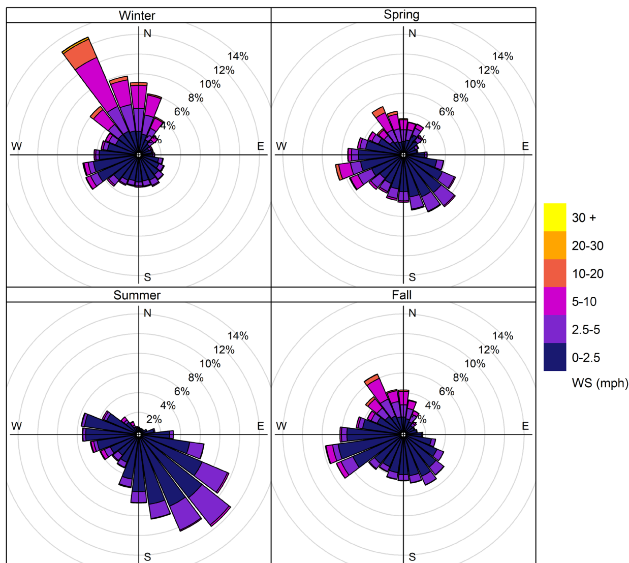
Figure B-5. Seasonal wind roses based on hourly data collected at the Community site from 2007-2025. Data from Year 11 to Year 16 are replaced with wind data from the Reseda site.
