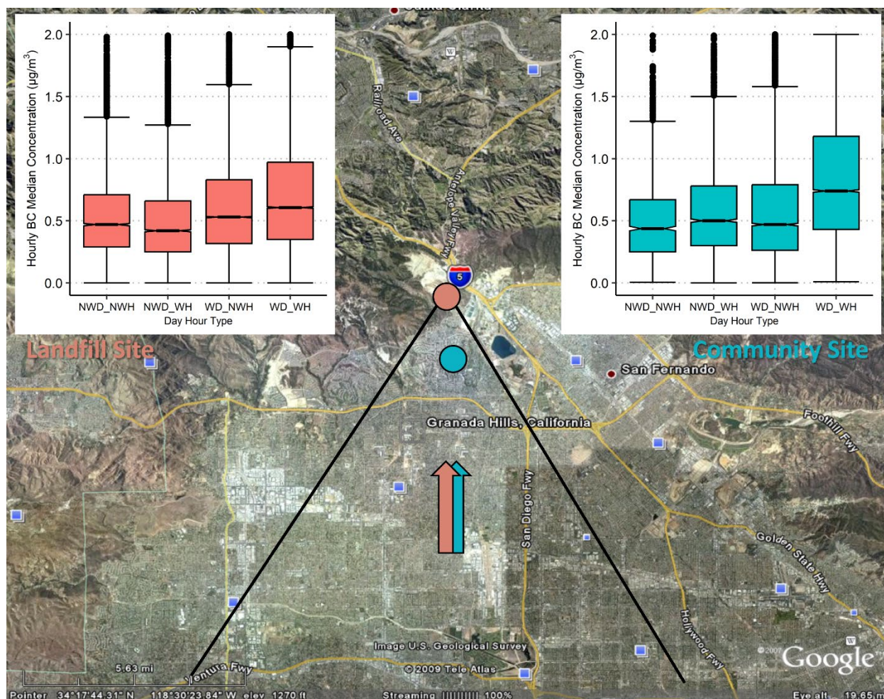
Figure 5-17. Notched box whisker plots of 18-yr hourly average BC concentrations for southerly ("From SoCAB") wind sectors (as displayed in Figure 5-5) for working days (WD), non-working days (NWD), working hours (WH), and non-working hours (NWH) within those days for the Landfill (red) and Community (blue) monitor sites. Outliers over 2 \mu\text{g}/\text{m}^3 are not displayed.
