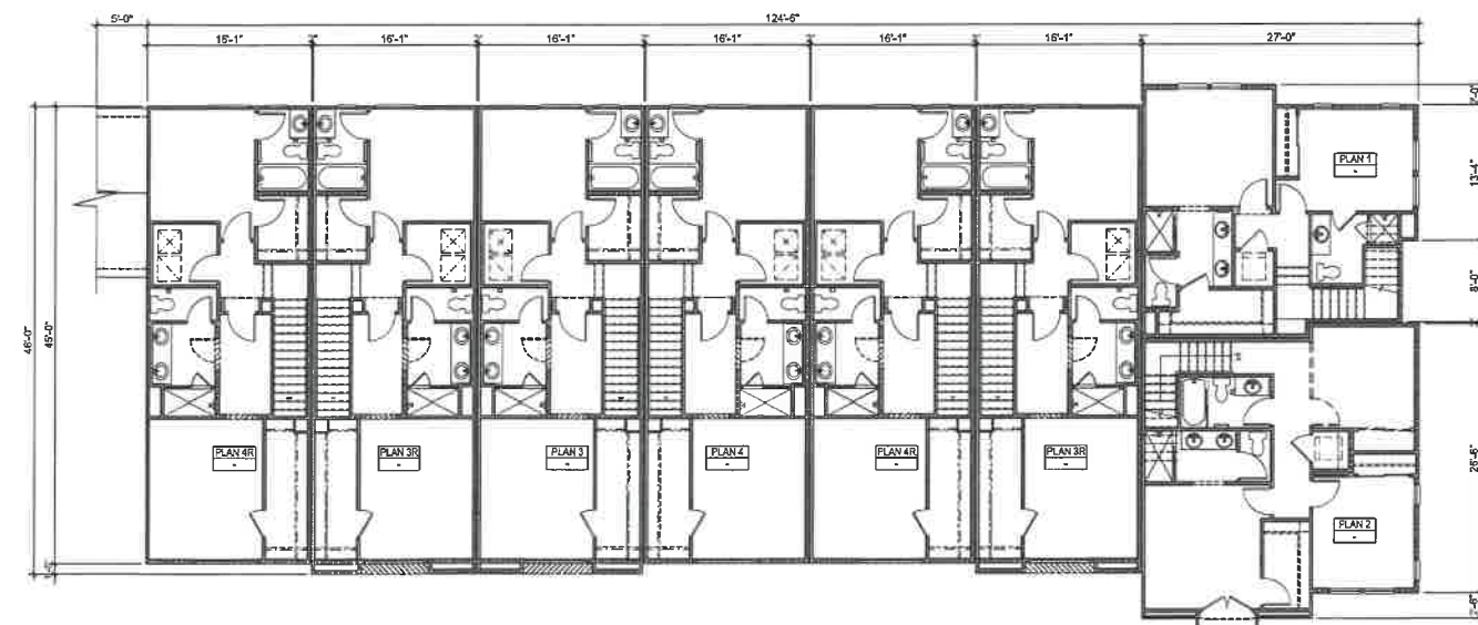
THIRD FLOOR
