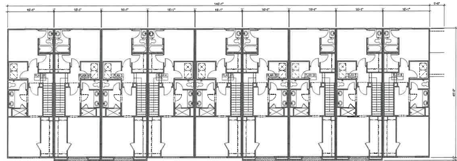
THIRD FLOOR
