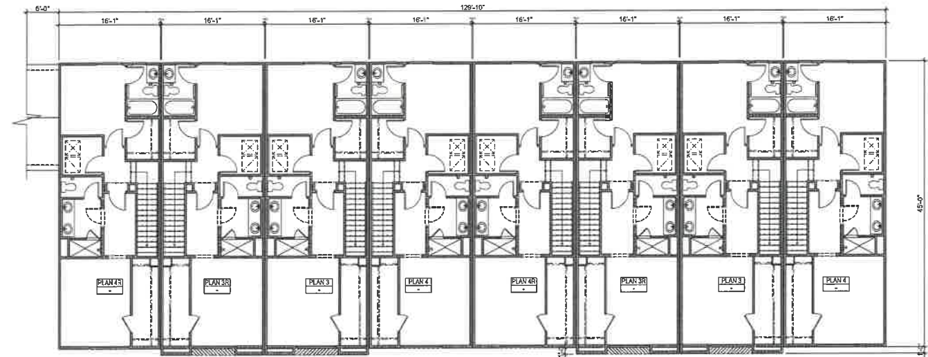
THIRD FLOOR
