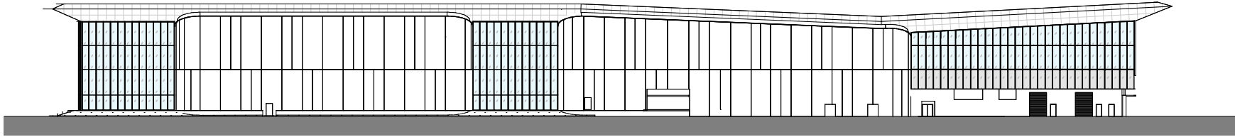
FUTURE CONCOURSE 0 ELEVATION - EAST
