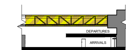
TYP TERMINAL PEDESTRIAN BRIDGE @ T1 & T7
