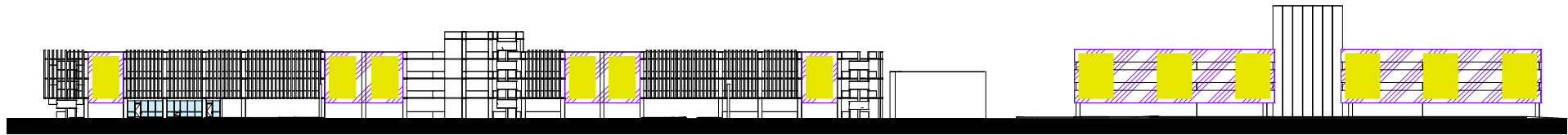
PARKING 2A ELEVATIONS - NORTH
