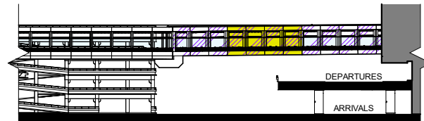
APM TERMINAL PEDESTRIAN BRIDGE - T3
