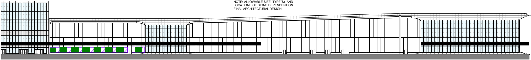
FUTURE CONCOURSE 0 ELEVATION - SOUTH
